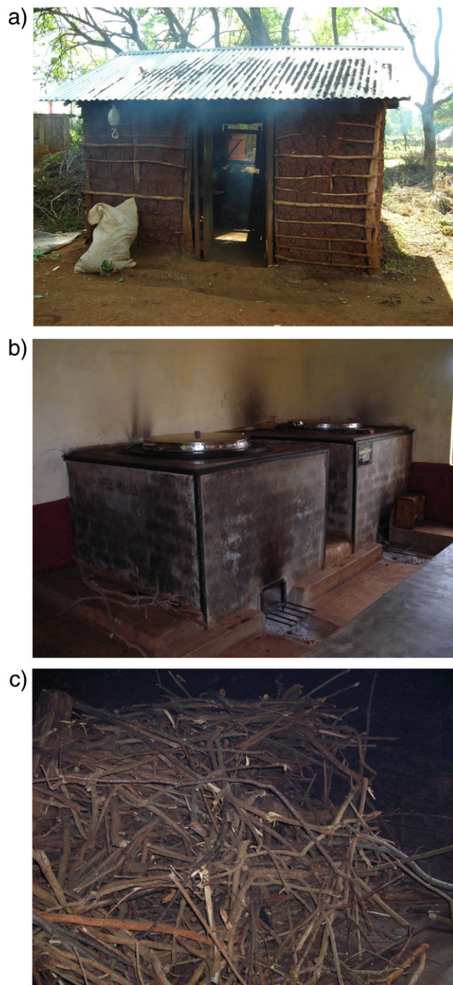
Fig. 1. Three images from Sauri village, Kenya: a) mud kitchen at Bar Tuoro Primary; b) Institutional Rocket Stove in a masonry kitchen, Nyamninia Primary; c) fuelwood in dry storage.
